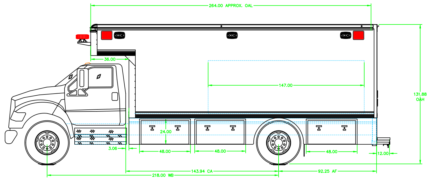
DRIVERSIDE VIEW
