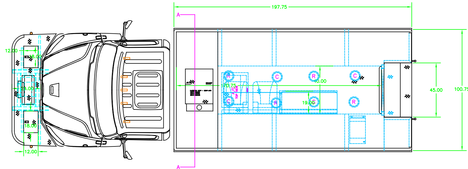
TOP VIEW
