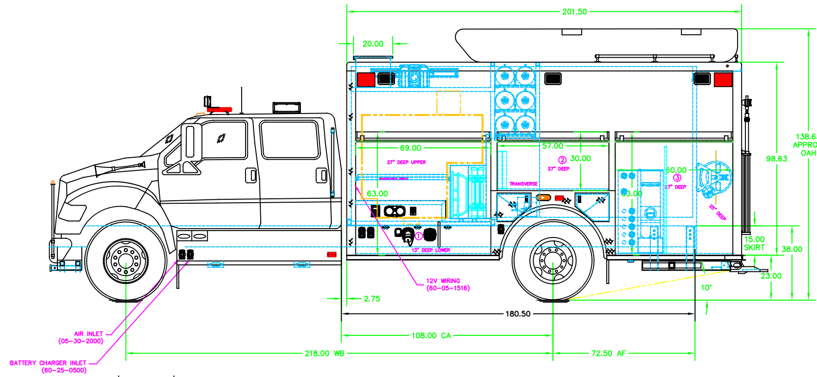
DRIVERSIDE VIEW
