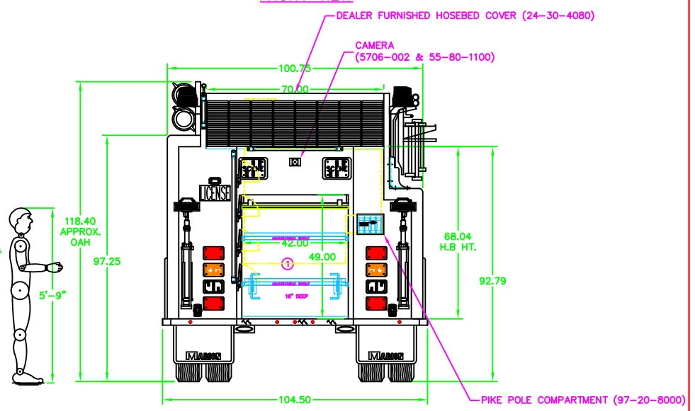
REAR VIEW
