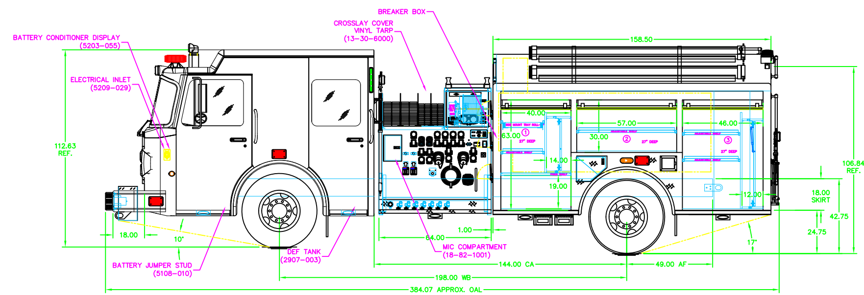
DRIVERSIDE VIEW
