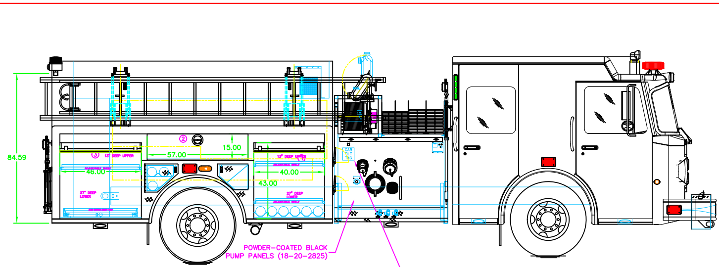
CURBSIDE VIEW CAB TILT (05-34-7500 & 2305-003)
