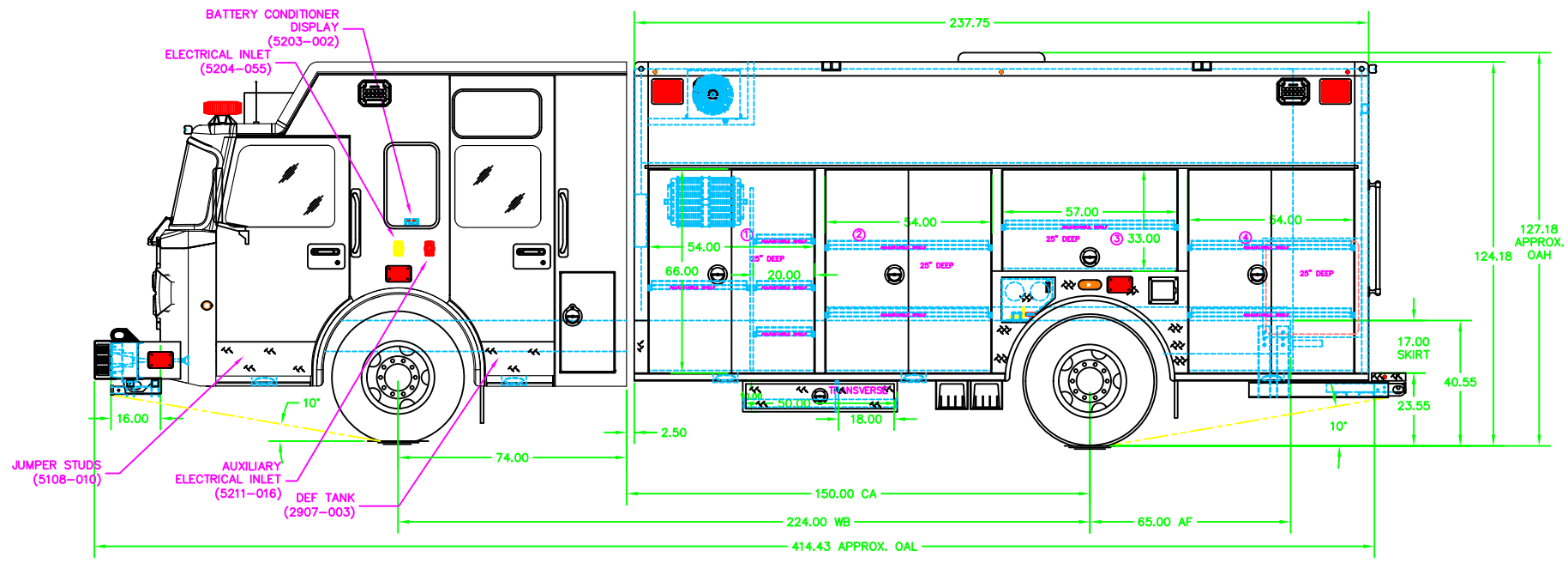
DRIVERSIDE VIEW
