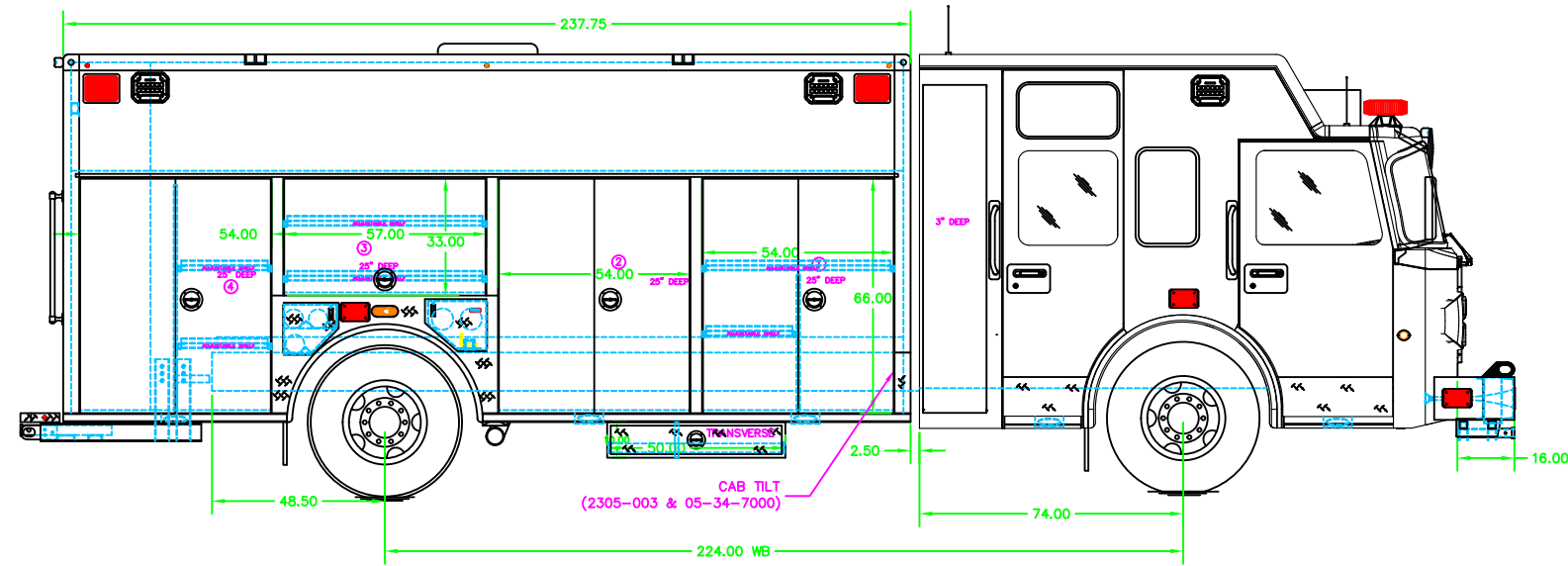
CURBSIDE VIEW
