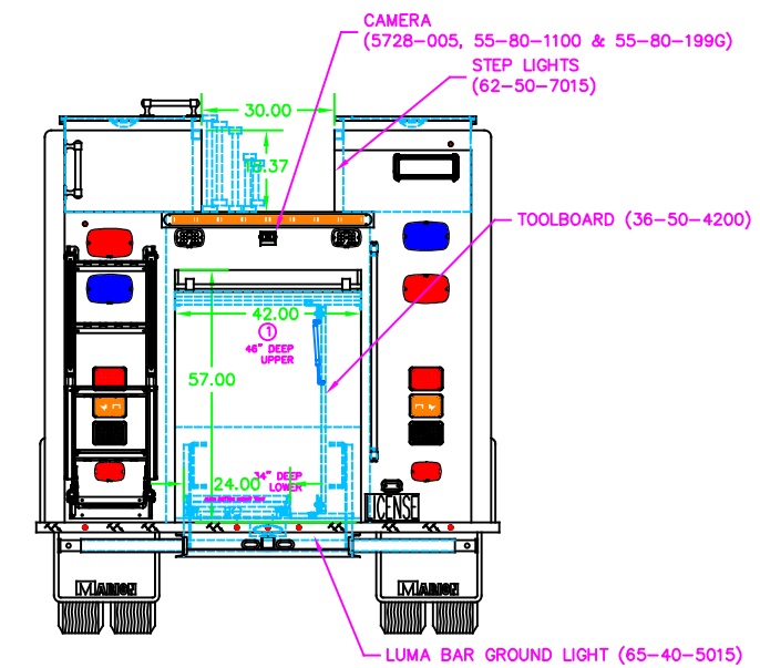
REAR VIEW
