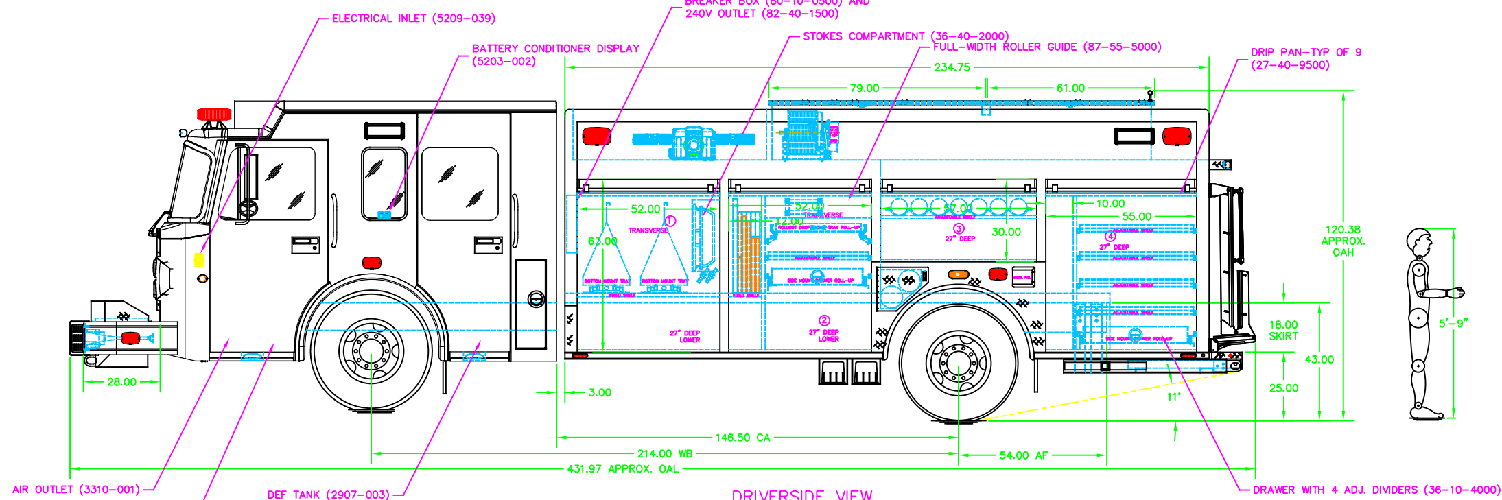
DRIVERSIDE VIEW
