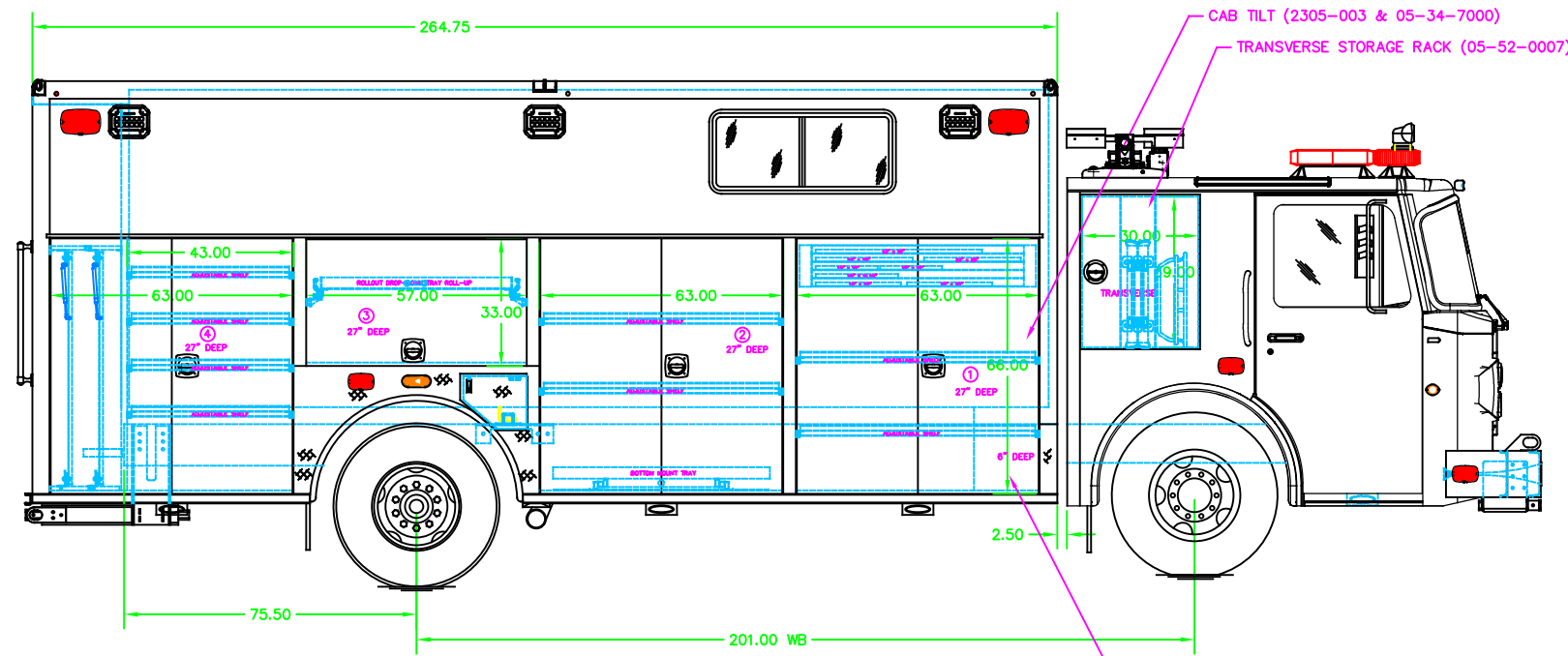
CURBSIDE VIEW
