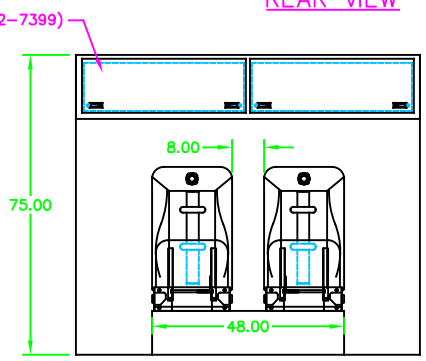
CAB CABINET (05-52-7399) (ALL DIMENSIONS APPROXIMATE)
