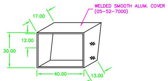
CAB CABINET (05-52-7000) (ALL DIMENSIONS APPROXIMATE)
