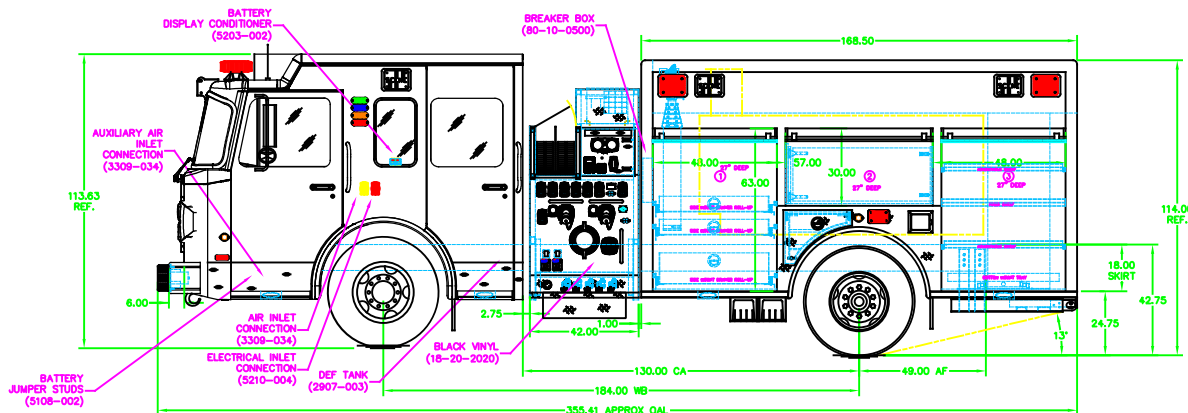
DRIVERSIDE VIEW
