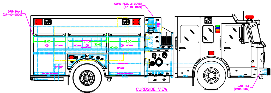
CURBSIDE VIEW
